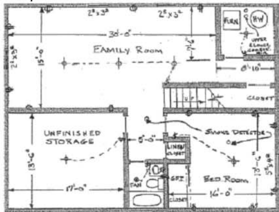
Sample Floor
